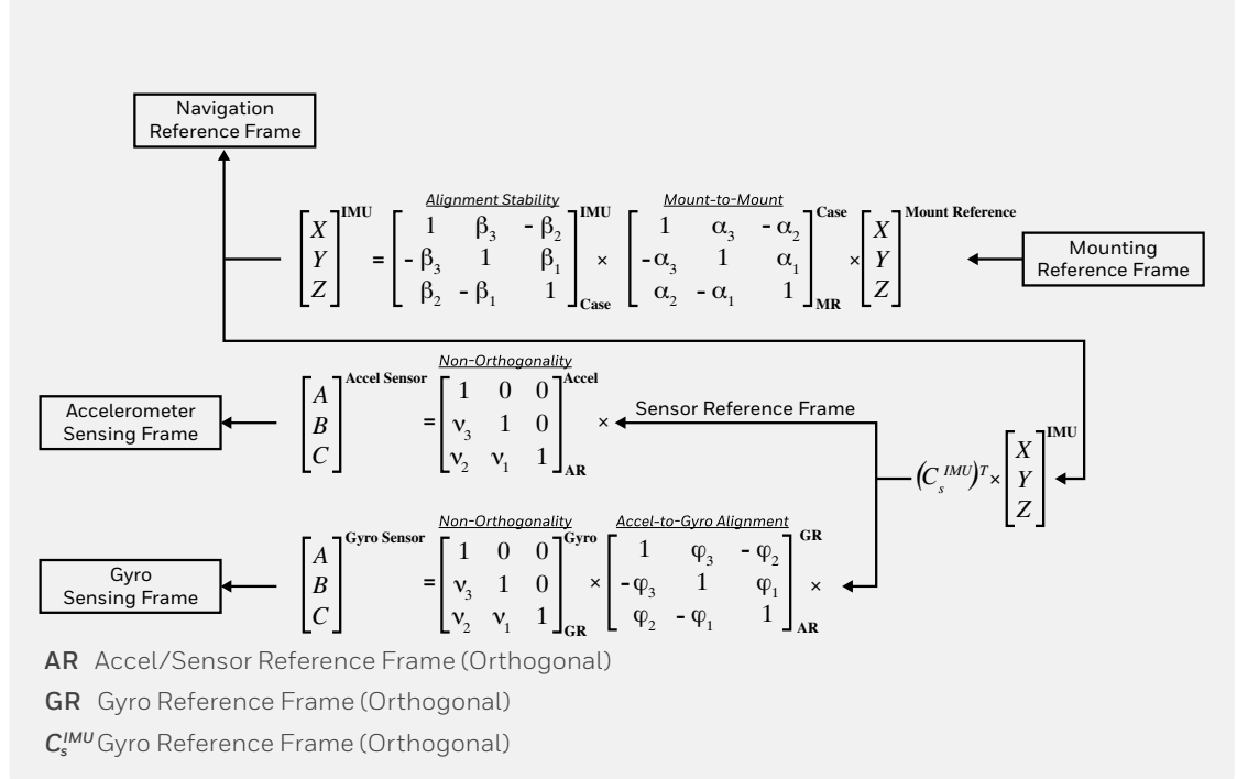
Figure 1. IMU Alignment Model
