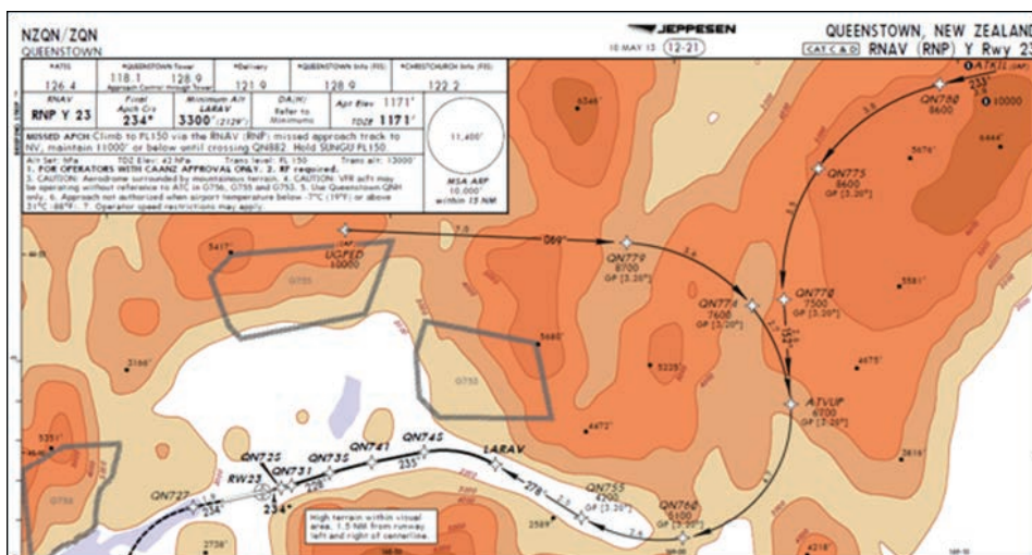
Fig. 3. RNAV RNP Approach with RF Legs
